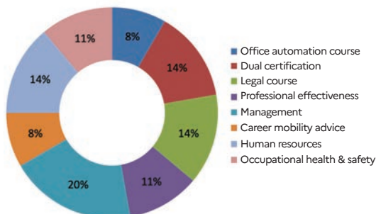
Training
